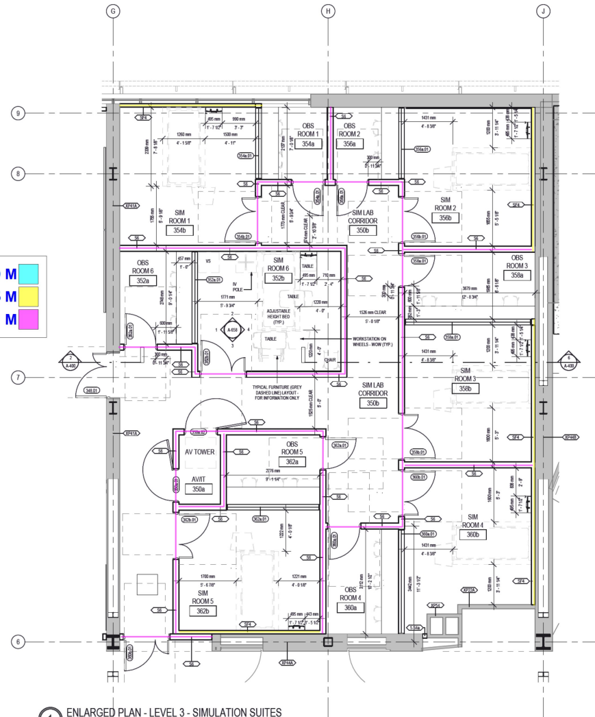
1 ENLARGED PLAN - LEVEL 3 - SIMULATION SUITES 1:50
