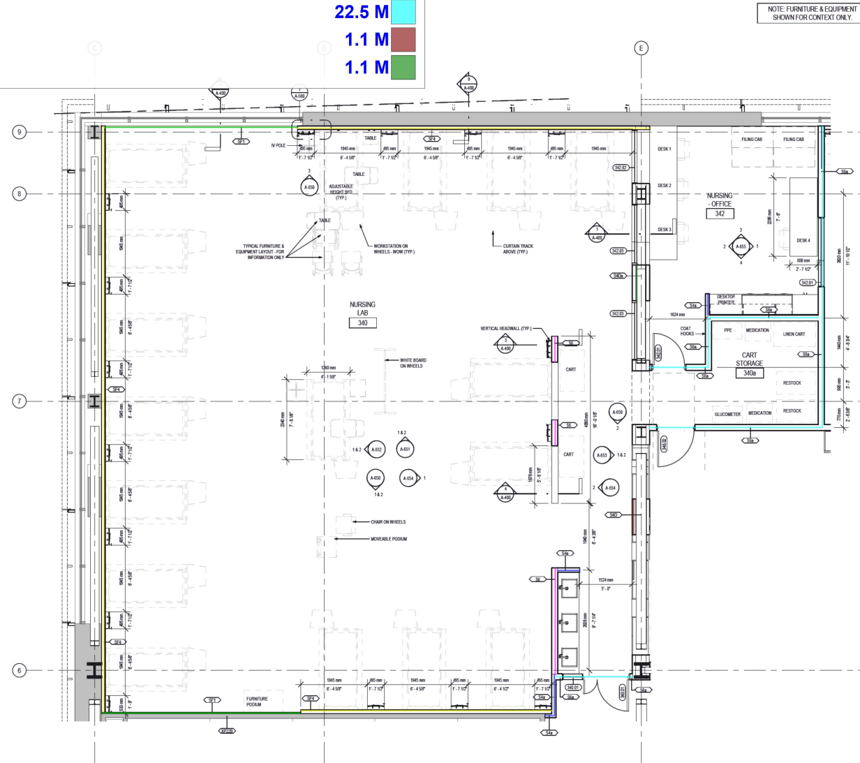
1 ENLARGED PLAN - LEVEL 3 - NURSING LAB & OFFICE 1 : 50
