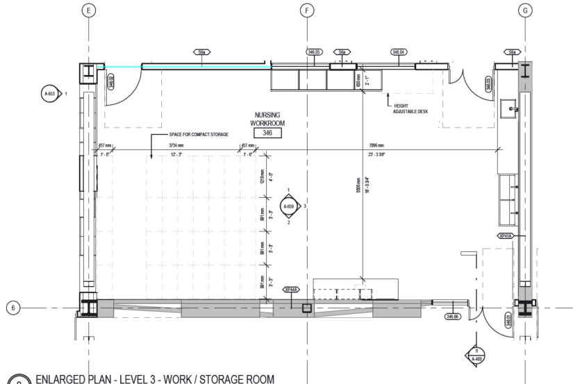
2 ENLARGED PLAN - LEVEL 3 - WORK / STORAGE ROOM 1:50
